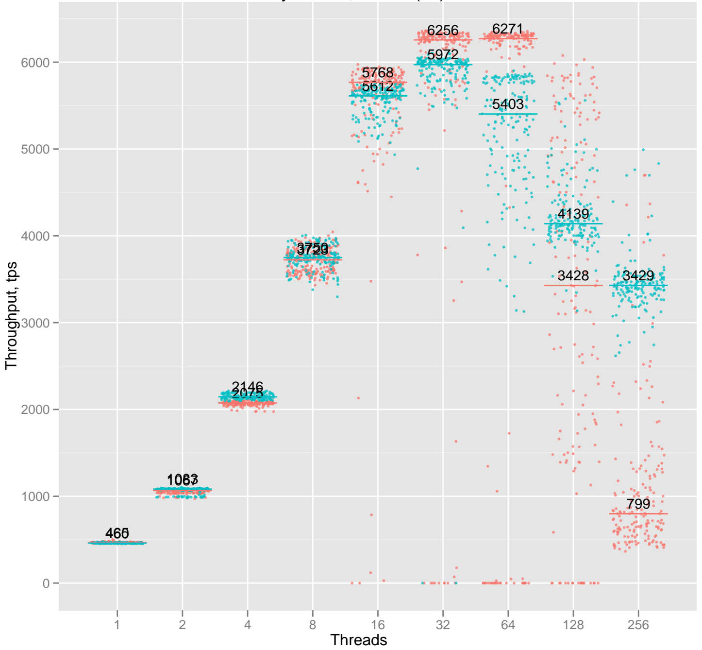
sysbench, OLTP (rw)
