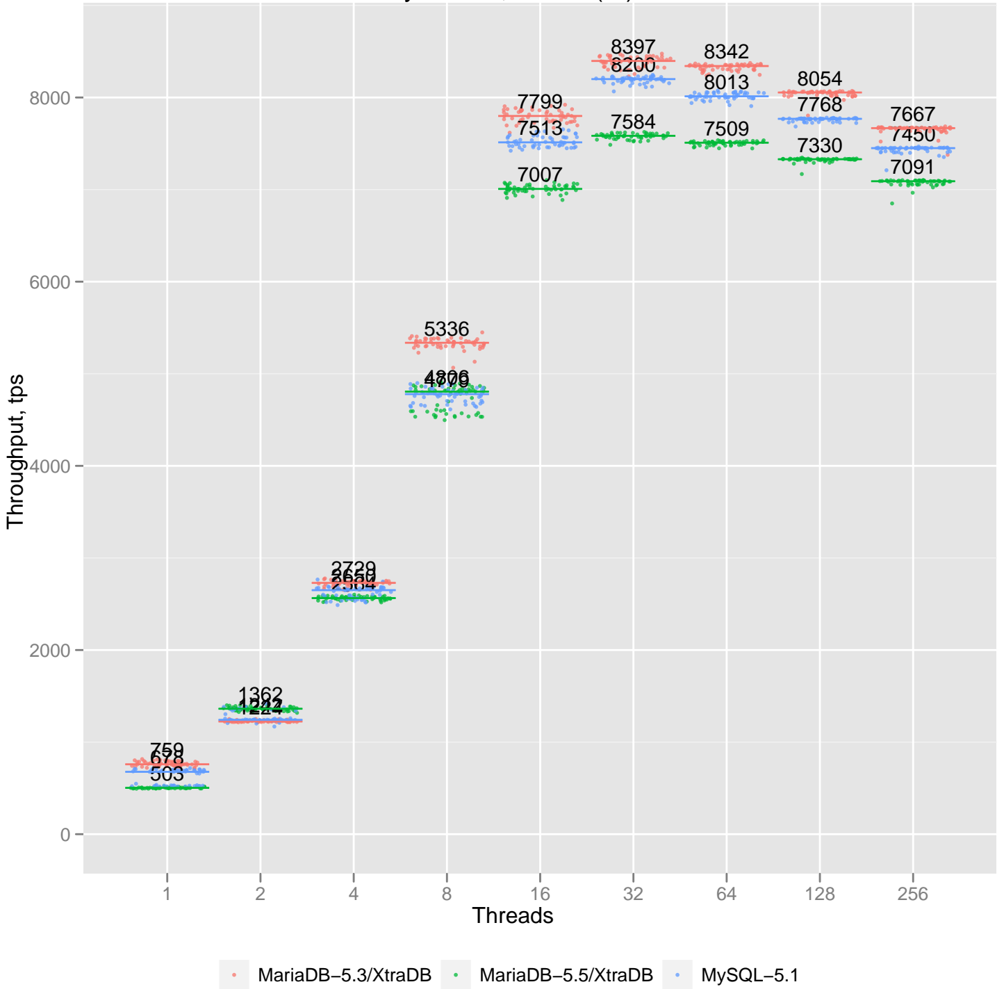
sysbench, OLTP (ro)
