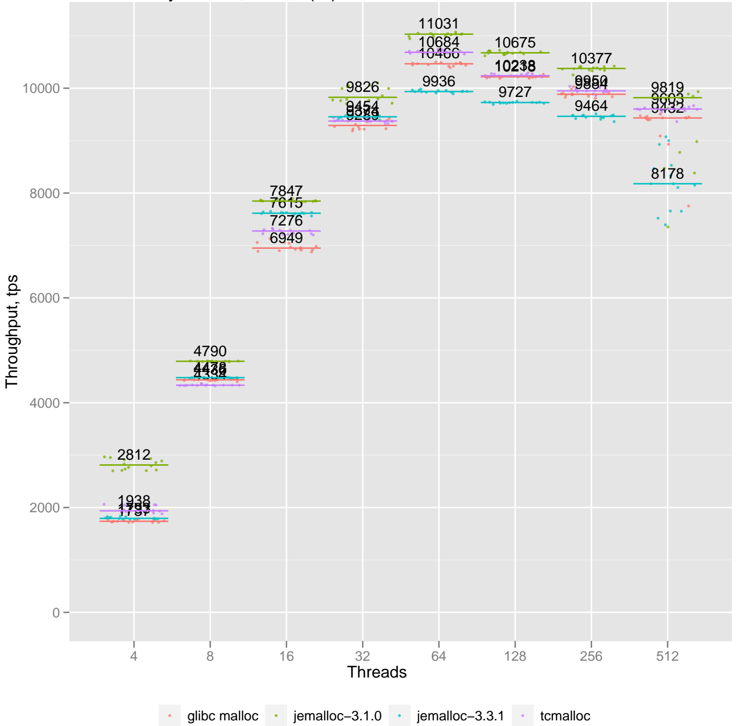
sysbench, OLTP (ro) MariaDB-5.5.30 vs. malloc lib
